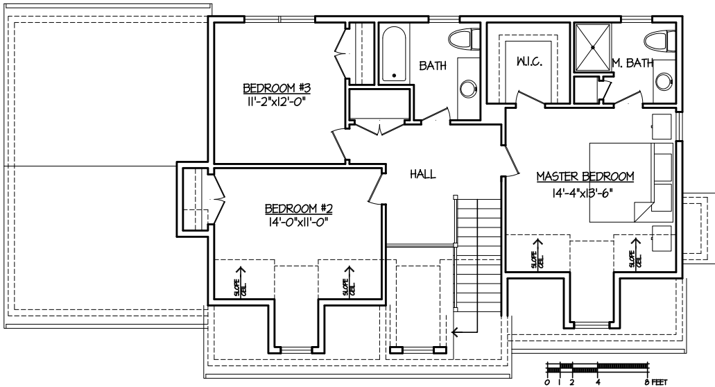
PROPOSED SECOND FLOOR 856 SQFT
