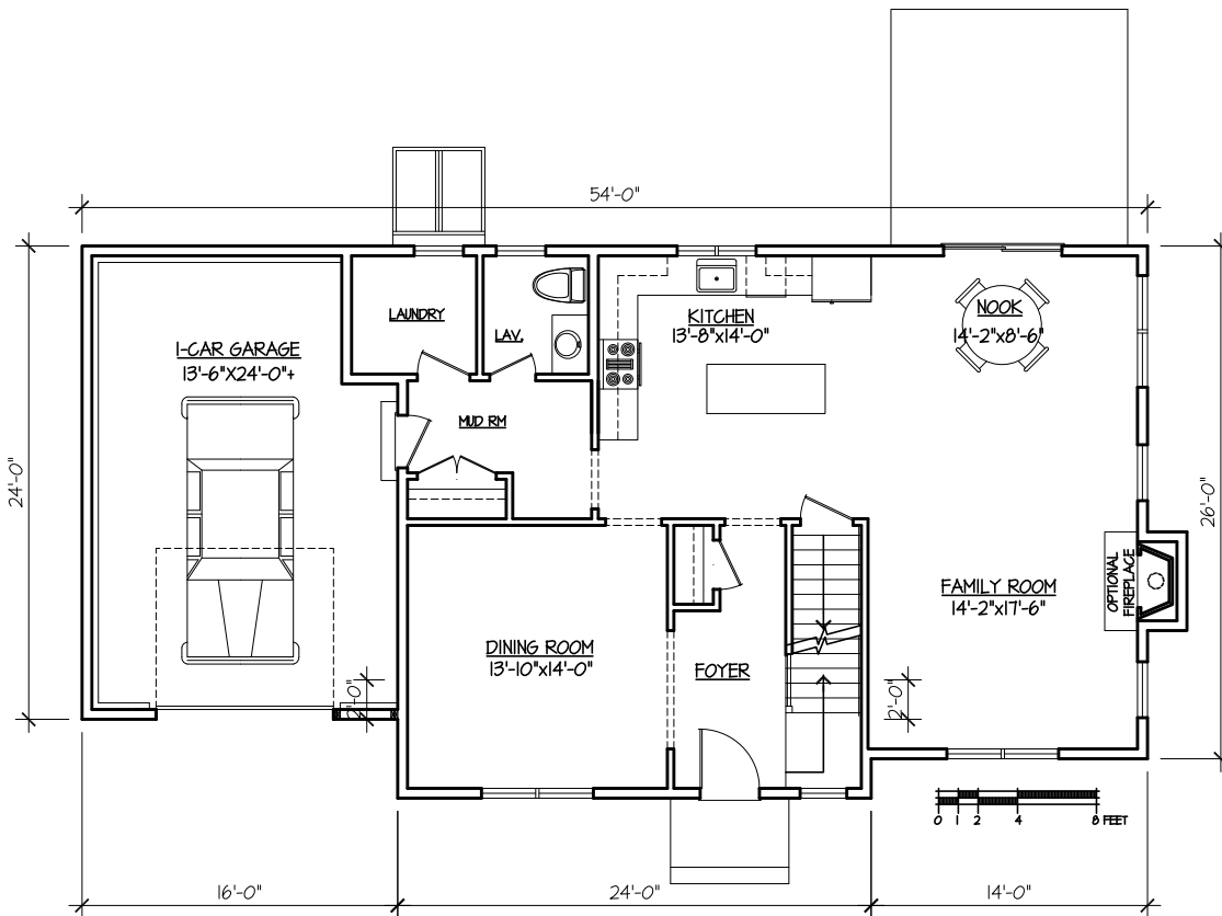
PROPOSED FIRST FLOOR 1056 SQFT
